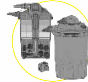
PF-30 PRESSURE FILTER WITH 11w UV LIGHT (Flow rate 4500L/H)
